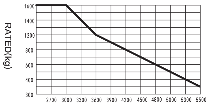
ES16-RS LIFT HEIGHT(mm)
