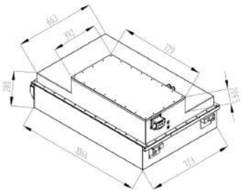
Dimension of lithium battery main box
