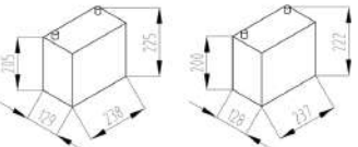
12V battery size
