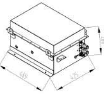
Dimension of lithium battery secondary box
